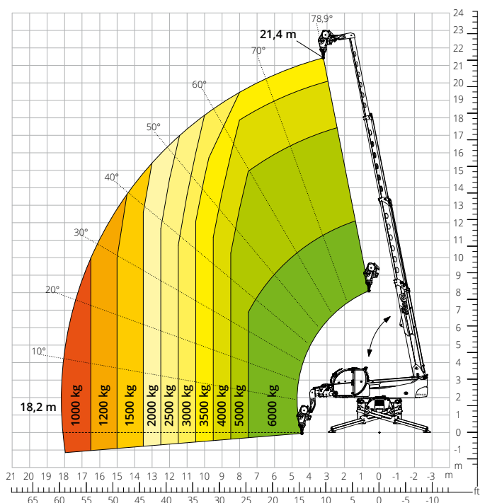
Load chart with WINCH, 6,000 kg ATT-02-004
