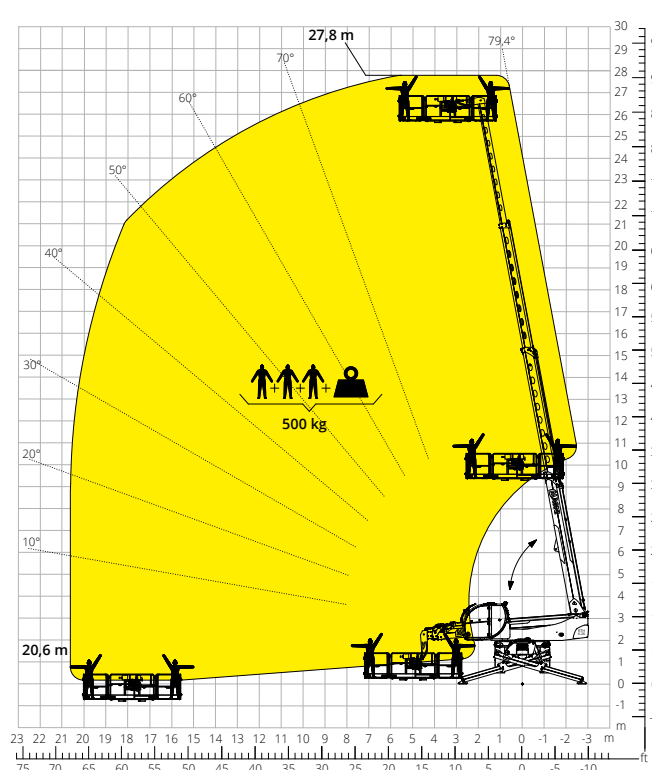
Load chart with ROTATING EXTENDABLE PLATFORM, 500 kg ATT - 01 - 005
